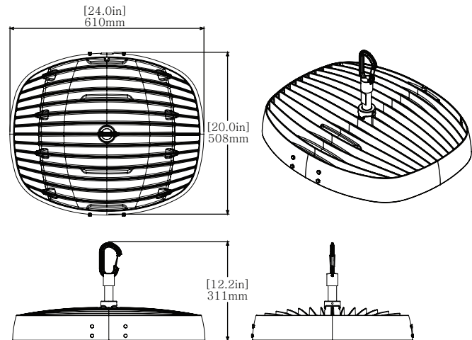
HOOKE PENDANT (AR-HK): 16.8 kg | 36.9 lbs
